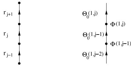
Fig. 2. Left: illustration of the returns involved in the ‘fitness’ criterion (17) (left), and the field components subject to updating (right), done at the ‘signal’ site j = j_s .
