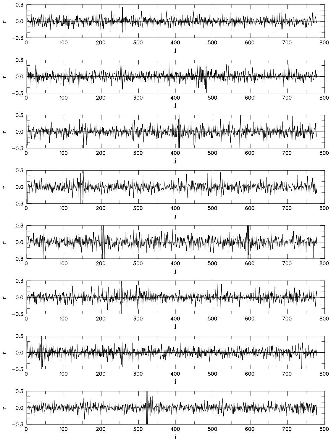
Fig. 9. Samples of returns time series for the update parameter \chi = 0013 . The corresponding gains distribution is shown in Fig. 7.
