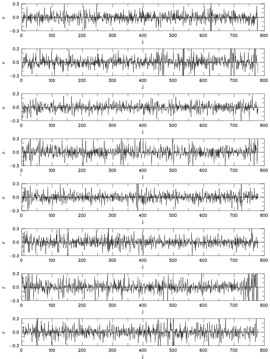
Fig. 8. Samples of returns time series for the update parameter \chi = 0005 . The corresponding gains distribution is shown in Fig. 7.
