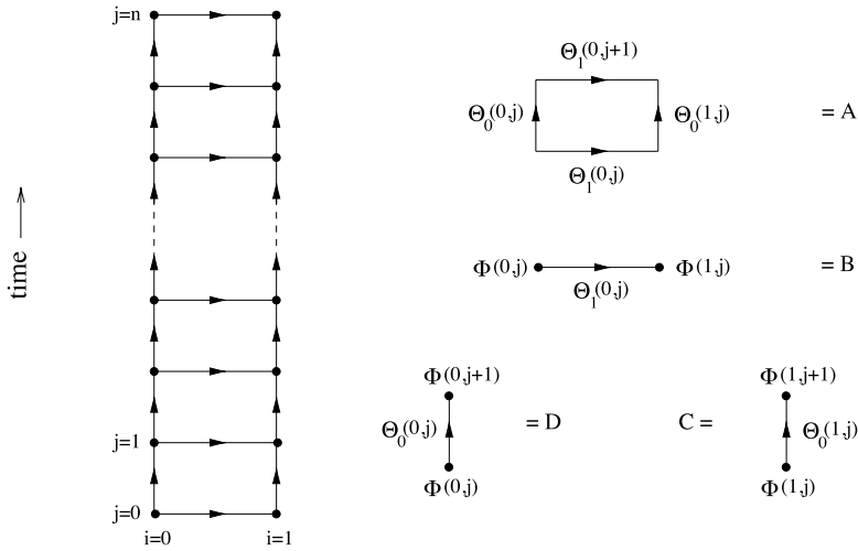
Fig. 1. Left: illustration of the ladder geometry of the lattice model and the label scheme for the fields. Right: depiction of the gauge invariant elements A, B, C, D used in the action.
