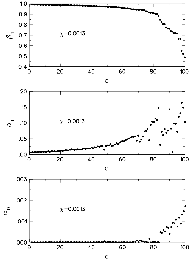
Fig. 11. GARCH(1, 1) fit parameters for a sample of 100 lattice time series at \chi = 0.0013 . The configuration counter c has been subject to sorting with respect to \beta_1 .
