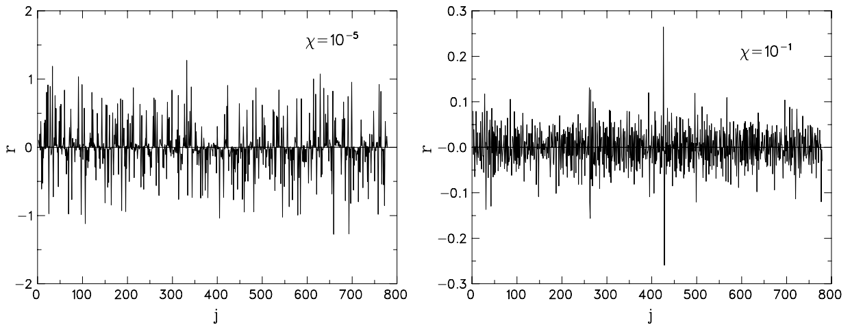
Fig. 6. Examples of returns time series r_j versus the lattice time j at \chi = 10^{-5} and \chi = 10^{-1} .
