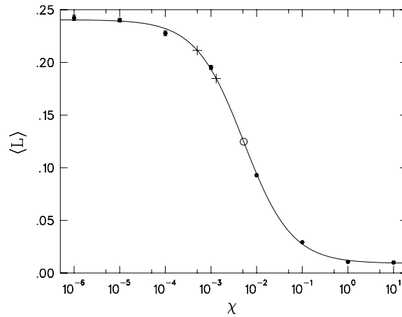
Fig. 3. Expectation value \langle L \rangle of the gauge invariant average link operator (29) as a function of the update parameter \chi in (24). The plotting symbols ‘•’ and ‘+’ correspond to specific values of \chi for which simulations were made. The symbol ‘o’ indicates the symmetry point \chi = 0.0052 of the fit.
