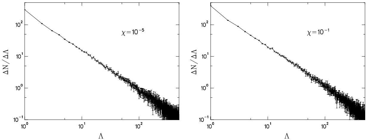
Fig. 4. Frequency distributions of avalanche sizes for two values \chi = 10^{-5}, 10^{-1} of the update parameter.
