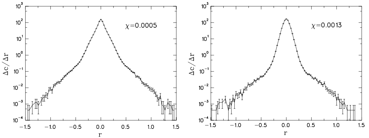
Fig. 7. Gains distributions from simulations with update parameter \chi = 0.0005 and \chi = 0.0013 .
