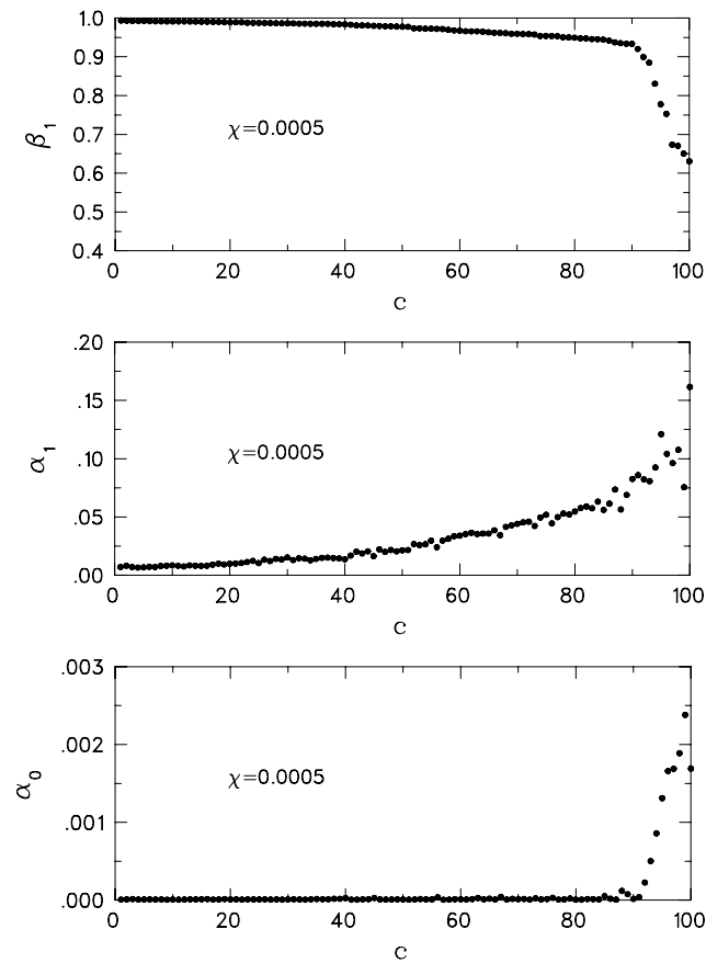
Fig. 10. GARCH(1, 1) fit parameters for a sample of 100 lattice time series at \chi = 0.0005 . The configuration counter c has been subject to sorting with respect to \beta_1 .
