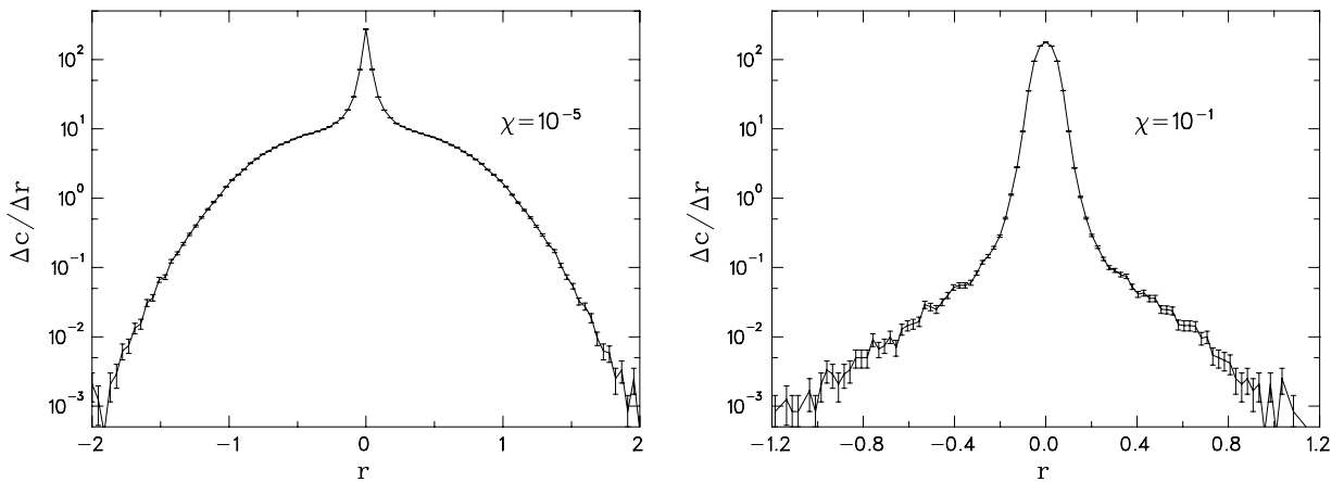
Fig. 5. Lattice generated gains distributions of the returns r for the values \chi = 10^{-5} , 10^{-1} of the update parameter.
