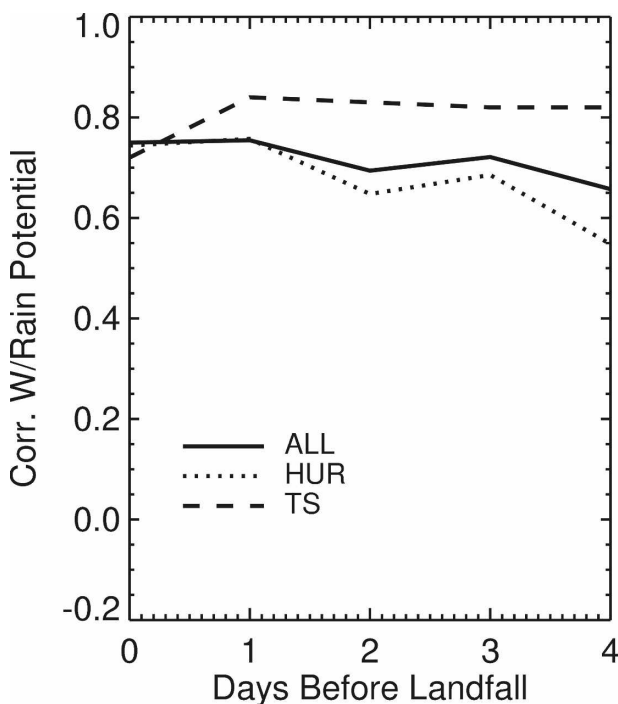
FIG. 7. Correlations between the maximum storm total rain over land and rainfall potential for 0–4 days before landfall for all tropical cyclones, HUR only, and TS only. HUR and TS represent the storm stage during landfall. The maximum storm total rain over land and rainfall potentials are in logarithmic scale.
