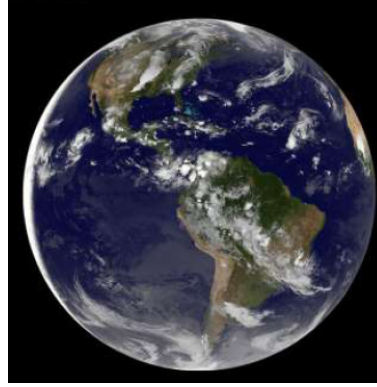
GOES-East
