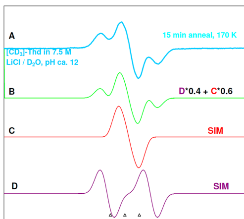
Figure 7. (A) The experimentally recorded (77 K) T(6OH) \cdot spectrum (thick sky blue, also in Figure 6B) obtained in the glassy (7.5 M LiCl/ D_2O ) sample of [CD_3] -dThd sample (3 mg/mL) in the presence of the electron scavenger K_2S_2O_8 at pH ca. 12, \gamma -irradiated to a dose of 1.4 kGy and progressively annealed to 170 K for 15 min. (B) Spectrum T(6OH) \cdot (green) due to addition of 60% of spectrum (C) to 40% of spectrum (D). (C) Simulated T(6OH) \cdot spectrum (red) using the parameters: HFCC values of 3 methyl deuterons 3.2 G and of C6-H 9 G, g = 2.0035 along with a mixed Lorentzian/Gaussian (1/1) line width of 6 G. These couplings are those expected from Table 1 and are unresolved. They only affect the line shape. (D) Simulated T(6OH) \cdot spectrum (violet) using the parameters: HFCC values of 3 methyl deuterons 3.2 G and of C6-H 39 G, g = 2.0035 along with a mixed Lorentzian/Gaussian (1/1) line width of 8 G. Here only the 39 G coupling is resolved.
