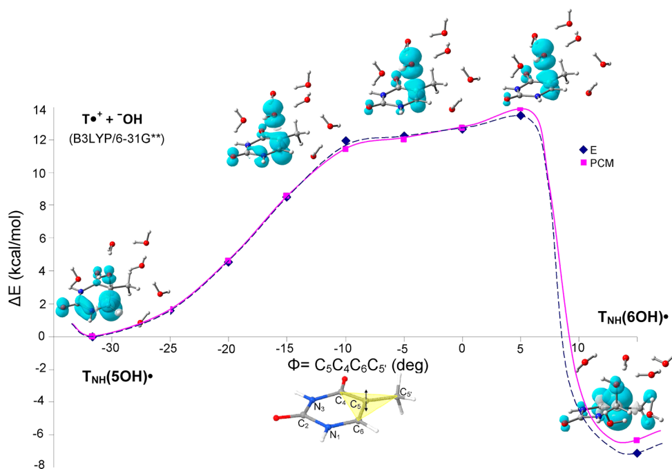
Figure 12. B3LYP/6-31G** calculated potential energy surface for the OH transfer from C5 to C6 atoms of hydrated T_{NH}(SOH)^\bullet with respect to the change of dihedral angle \Phi ( C_5-C_4-C_6-C_5' ) of thymine ring. The structures at the beginning (ca. -32^\circ ) and end (ca. 15^\circ ) are fully optimized. The up and down arrows at C5 show the movement of C5 atom with respect to C4, C6, and C5' atoms. The energies (kcal/mol) were calculated in the gas phase (blue \blacklozenge ) and in PCM (magenta \blacksquare ). The variation of spin density distribution along the PES is also shown at some chosen points, for details see Supporting Information Table T1.
