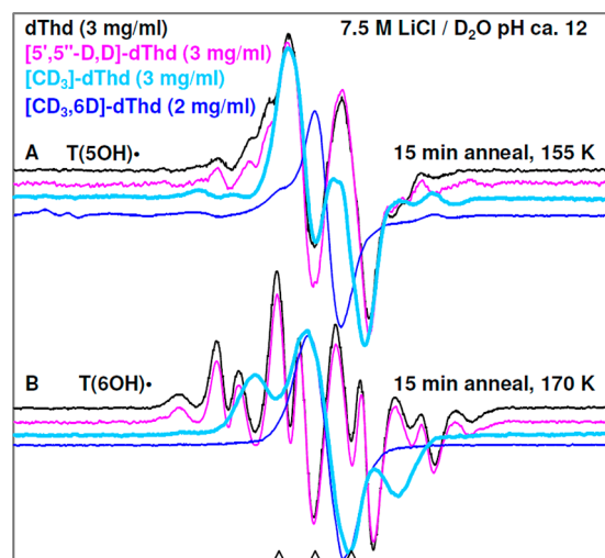
Figure 6. ESR spectra obtained from dThd (black), [5',5''-D,D] -dThd (pink), [CD_3] -dThd (thick sky blue), and [CD_3,6D] -dThd (blue). These samples were prepared identically [concentration = 2 to 3 mg/mL, in the presence of the electron scavenger K_2S_2O_8 at pH ca. 12], \gamma -irradiated to a dose of 1.4 kGy. (A) Spectra of T(SOH)\cdot obtained via annealing to 155 K for 15 min. (B) Spectra of T(6OH)\cdot obtained after annealing each sample to 170 K for 15 min.
