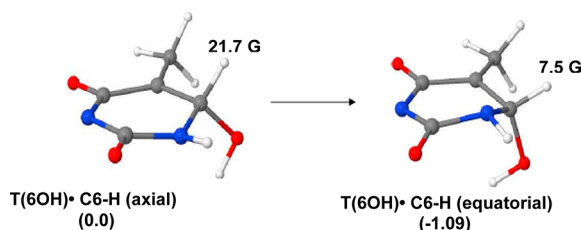
Figure 13. B3LYP/6-31G** fully optimized conformations of T(6OH)\cdot (C6–H axial) and T(6OH)\cdot (C6–H equatorial) in the gas phase with thymine base deprotonated at N3. The relative stabilities of the two conformers of T(6OH)\cdot in kcal/mol are provided in parentheses.
