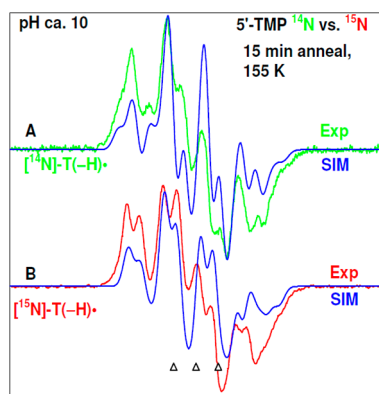
Figure 1. ESR spectrum of T(-H)• formed via annealing at 155–160 K after one-electron oxidation of the thymine base by \text{Cl}_2^{\bullet-} in aqueous glassy sample of (A) unlabeled 5'-TMP, green color, and of (B) ^{15}\text{N} labeled 5'-TMP, red color. The simulated spectra (blue) (for simulation parameters, see text) are superimposed on the top of the each experimentally recorded spectrum.
