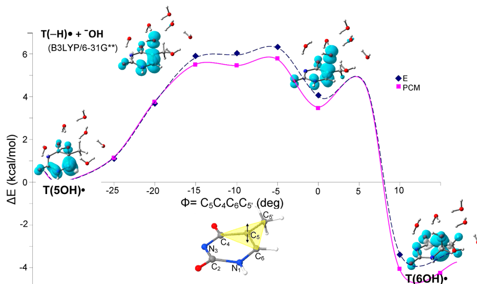
Figure 11. B3LYP/6-31G** calculated potential energy surface for the OH transfer from C5 atom to the C6 atom in the thymine base of hydrated \text{T(5OH)}^\cdot with respect to the change of dihedral angle \Phi ( \text{C}_5\text{--C}_4\text{--C}_6\text{--C}_5' ) of thymine ring. The structures at the beginning (ca. -32^\circ ) and end (ca. 16^\circ ) are fully optimized. The up and down arrows at C5 show the movement of C5 atom with respect to C4, C6, and \text{C}_5' atoms. The energies (kcal/mol) were calculated in gas phase (blue \blacklozenge ) and in PCM (magenta \blacksquare ). The variation of spin density distribution along the PES is also shown at some chosen points (see Supporting Information Table T1).
