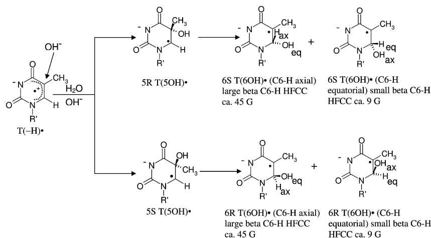
Scheme 4. Addition of \text{OH}^- to C5 of \text{T}(-\text{H})\cdot Yields \text{T}(\text{SOH})\cdot (5R and/or 5S) a
