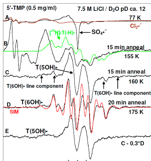
Figure 2. ESR spectra of (A) \gamma -irradiated glassy sample of 5'-TMP (0.5 mg/mL in 7.5 M LiCl/D 2 O) in the presence of electron scavenger \text{K}_2\text{S}_2\text{O}_8 at pH ca. 12 (black); partial spectrum (brown, 220 G scan) of a pure \text{Cl}_2^{\bullet-} spectrum is overlapped on the black spectrum in A to show the \text{Cl}_2^{\bullet-} line components in the black spectrum. (B–D) Spectra (black) found after annealing to (B) 155 K for 15 min, (C) 160 K for 15 min, (D) 175 K for 20 min. The spectrum of T(-H)• (green, Figure 1A) is overlapped on spectrum (B). The red spectrum in (D) is the simulated spectrum of T(6OH)• which is a mixture of T(6OH)• with \beta C6–H HFCC of 9 G (80%) and with \beta C6–H HFCC of 45 G (20%). See text and Supporting Information Figure S2 for details of simulation. (E) The black spectrum, assigned to T(SOH)•, is obtained by 30% subtraction of spectrum (D) from spectrum (C). All spectra are recorded at 77 K.
