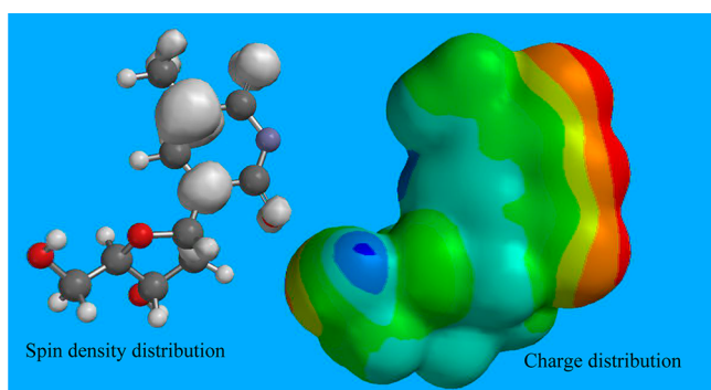
Figure 10. The optimized structure with spin densities and distribution of charge in \text{T(-H)}^\cdot of dThd calculated at the B3LYP/6-311++G**//B3LYP/6-31G* level in the gas phase. Red color region represents negative charge, whereas the blue color region represents positive charge distributions. The radical has considerable charge separation and is near zwitterionic in nature.
