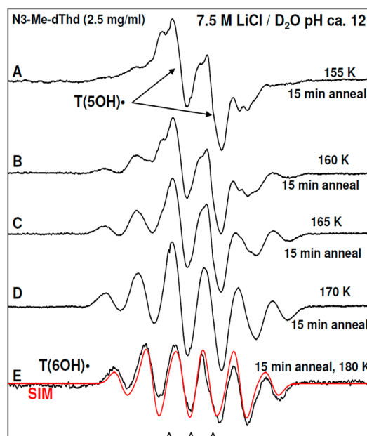
Figure 4. ESR spectra of (A) \gamma -irradiated glassy sample of N3\text{-Me-dThd} (2.5 mg/mL in 7.5 M \text{LiCl}/\text{D}_2\text{O} ) in the presence of electron scavenger \text{K}_2\text{S}_2\text{O}_8 at pH ca. 12 and annealed to 155 K for 15 min and the central doublet is assigned to T(\text{SOH})\cdot ; (B) 160 K for 15 min; (C) 165 K for 15 min; (D) 170 K for 15 min; (E) 180 K for 15 min. This spectrum is assigned to T(6OH)\cdot in the C6–H axial conformation (Scheme 4). The red spectrum is the simulated spectrum of T(6OH)\cdot using HFCC values of each of the 3 \beta methyl protons (19 G) with \beta C6–H HFCC of 33 G, line width 8 G, and g = 2.0035 .
